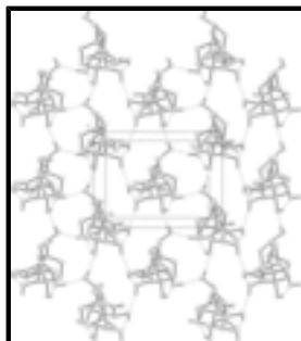
Fig. 2. A perspective view of the crystal packing of (I) showing the intermolecular hydrogen bonds as dashed lines.
