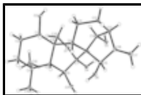
Fig. 1. Molecular configuration and atom numbering scheme for compound (I). Displacement ellipsoids are drawn at the 50% probability level.
